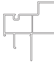
7358 INTEGRAL "J" CHANNEL WHITE - BV735801 ALMOND - BV735854 CLAY - BV735851
