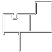
7818 7/8" NAIL FLANGE WHITE - BV781801 ALMOND - BV781854 CLAY - BV781851
