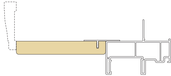
280/580 w/ 6 9/16" WOOD LINER
