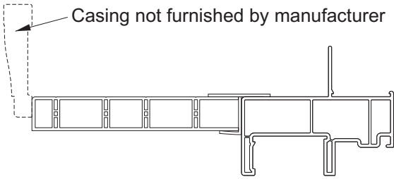
280/580 w/ 6 9/16" JAMB EXTENDER
