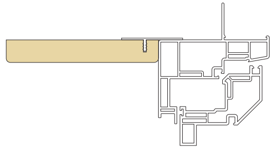
680 CASEMENT/AWNING w/ 6 9/16" WOOD LINER
