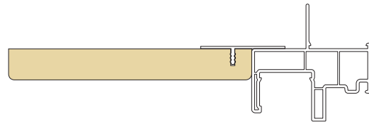
270/570 w/ 6 9/16" WOOD LINER
