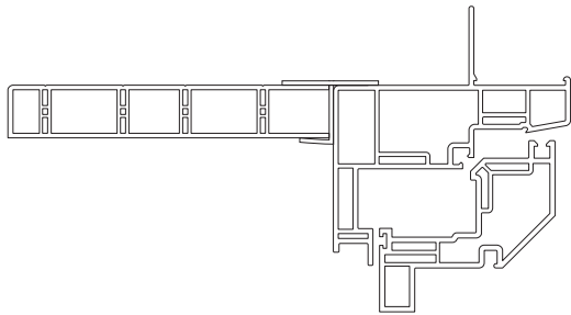
680 CASEMENT/AWNING w/ 6 9/16" JAMB EXTENDER
