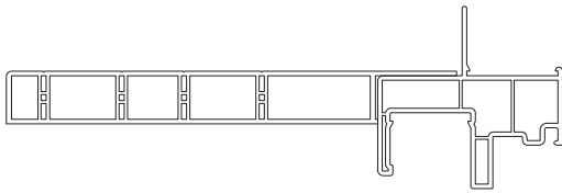
270/570 w/ 6 9/16" JAMB LINER
