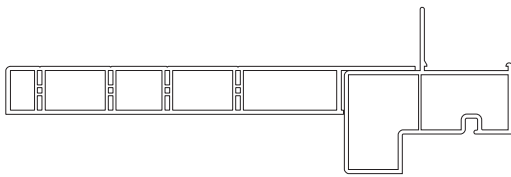
770 w/ 6 9/16" JAMB LINER
