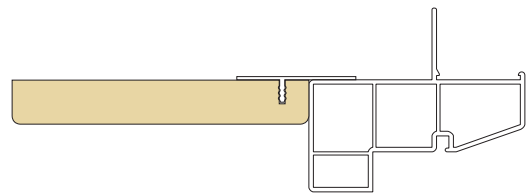
780 w/ 6 9/16" WOOD LINER
