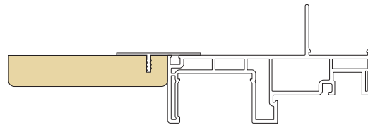
170 PD w/ 6 9/16" WOOD LINER
