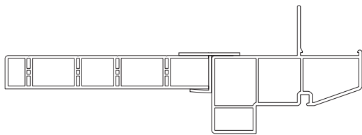
780 w/ 6 9/16" JAMB EXTENDER
