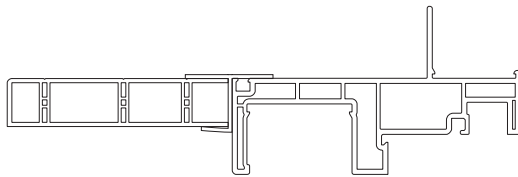
170 PD w/ 6 9/16" JAMB LINER
